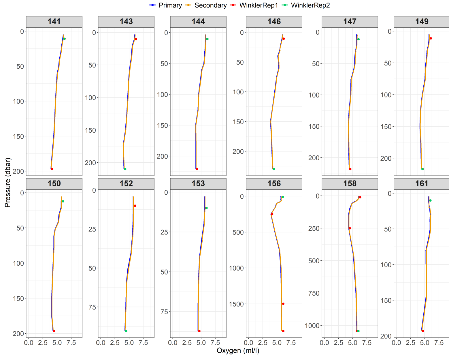
Figure A2.5: Relationship between primary (blue) and secondary (orange) dissolved oxygen sensors and dissolved oxygen measurements (replicate 1 = red, replicate 2 = green) from the Winkler titration method for Events 141 to 161.
