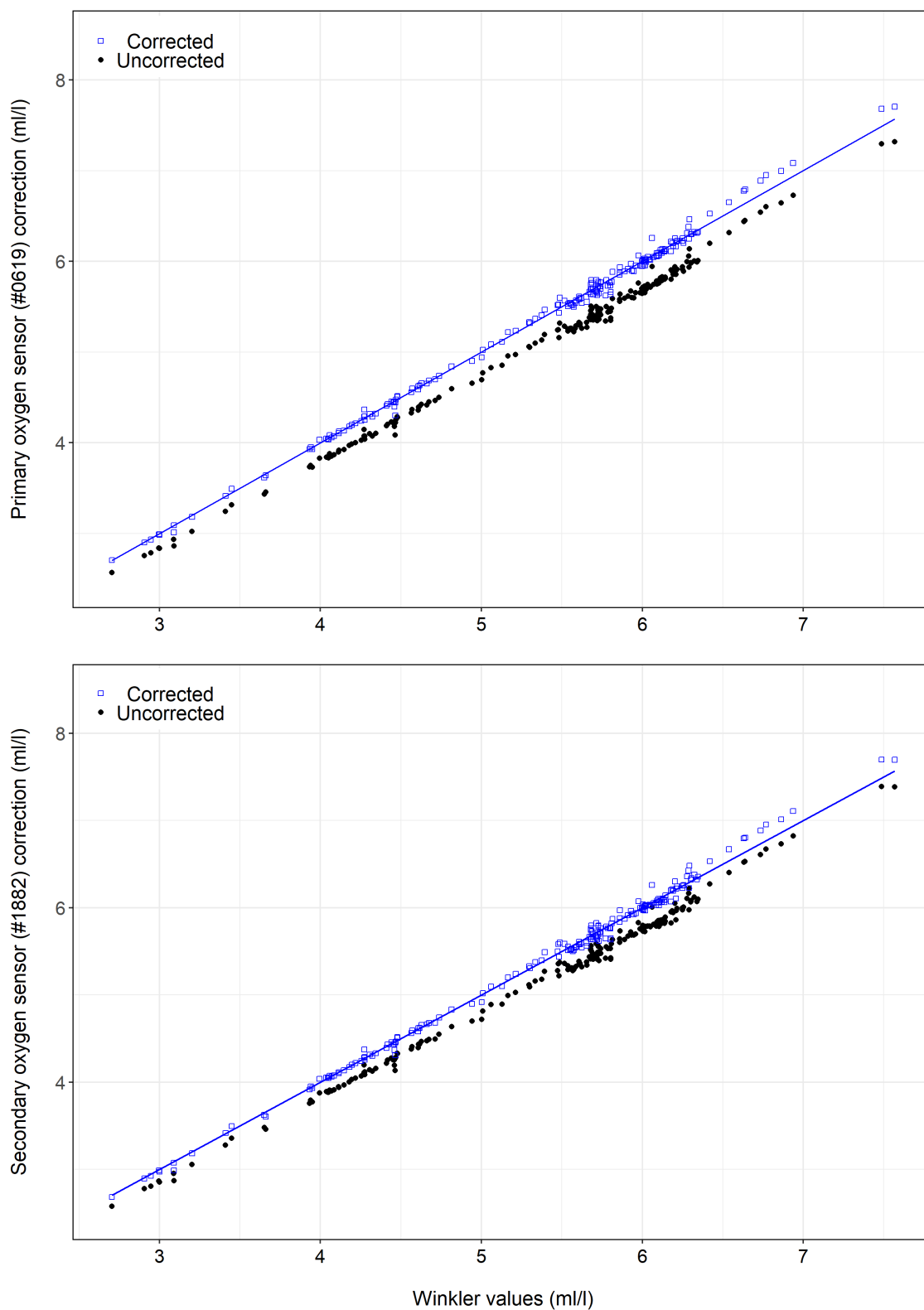
Figure A3.5: Primary (top) and secondary (bottom) oxygen sensor data before (black dots) and after (blue squares) correction using the slope correction ratio. The blue line represents the 1:1 reference line of the corrected data.
