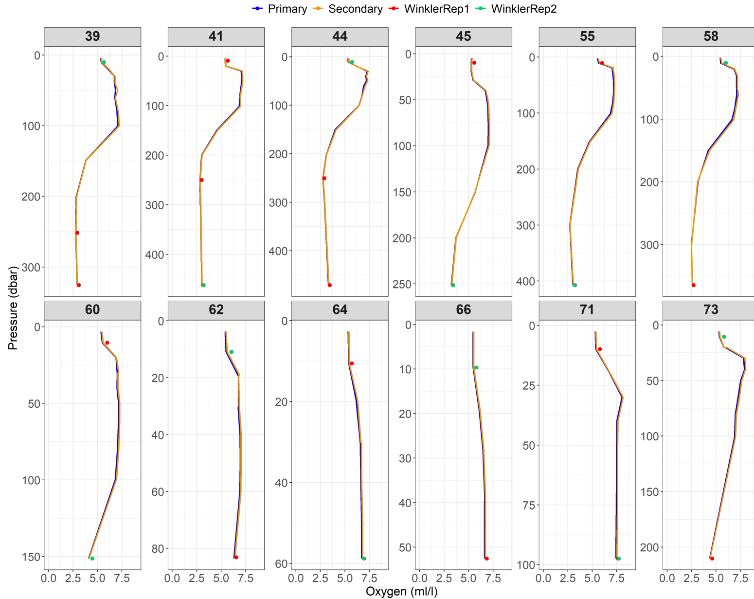
Figure A2.2: Relationship between primary (blue) and secondary (orange) dissolved oxygen sensors and dissolved oxygen measurements (replicate 1 = red, replicate 2 = green) from the Winkler titration method for Events 39 to 73.
