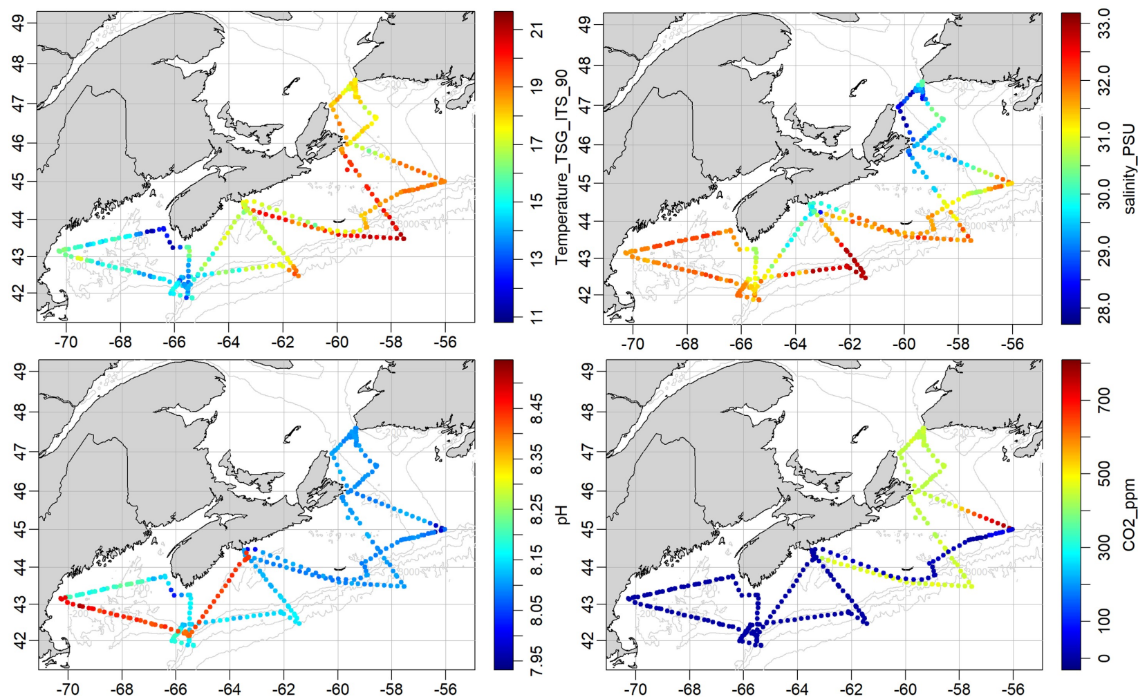
Figure 8: Surface temperature (°C; top left), salinity (PSU; top right), pH (lower left), and the partial pressure of carbon dioxide (pCO 2 ; lower right) measured along the cruise track during the 2023 Fall AZMP mission (DY16902). Data are measured at variable intervals and presented as hourly interpolations.
