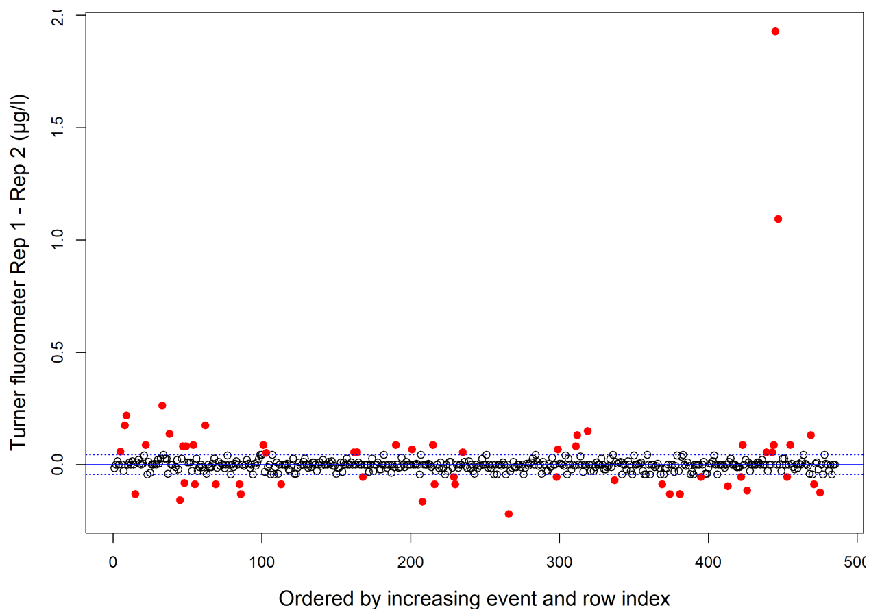
Figure A5.1: Comparison of Turner fluorometer replicates. Differences above or below the IQR min/max are considered outliers (red dots) and were removed from the evaluation process. Boxplot statistics are as follows: Median = 0.0000, IQR min = -0.0438, IQR max = 0.0438.
