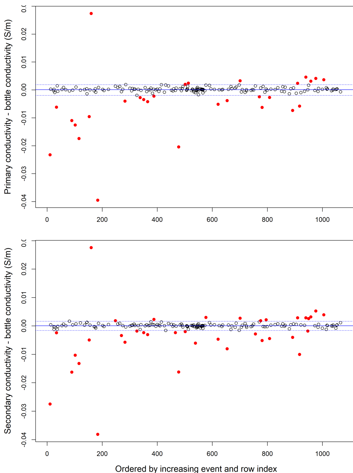
Figure A4.2: Comparison between primary (top) and secondary (bottom) conductivity sensor data and bottle conductivity (S/m) collected during the DY16902 mission. Differences outside 1.5 \times \text{IQR} (horizontal dashed blue lines) are considered outliers (red dots) and were removed from the calibration process. Boxplot statistics are as follows: A) Median = 0.0001, IQR min = -0.0019, IQR max = 0.0019; B) Median = 7.3414 \times 10^{-5} , IQR min = -1.6116 \times 10^{-3} , IQR max = 1.6451 \times 10^{-3} .
