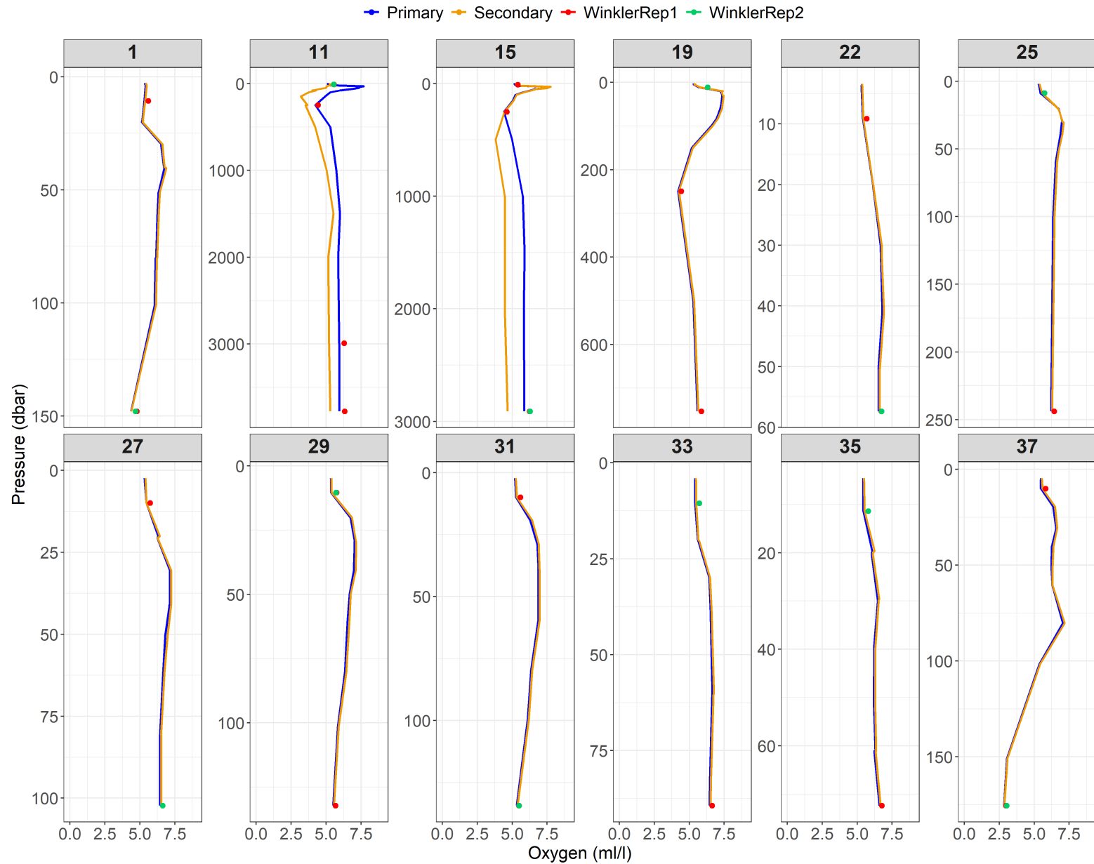
Figure A2.1: Relationship between primary (blue) and secondary (orange) dissolved oxygen sensors and dissolved oxygen measurements (replicate 1 = red, replicate 2 = green) from the Winkler titration method for Events 1 to 37.
