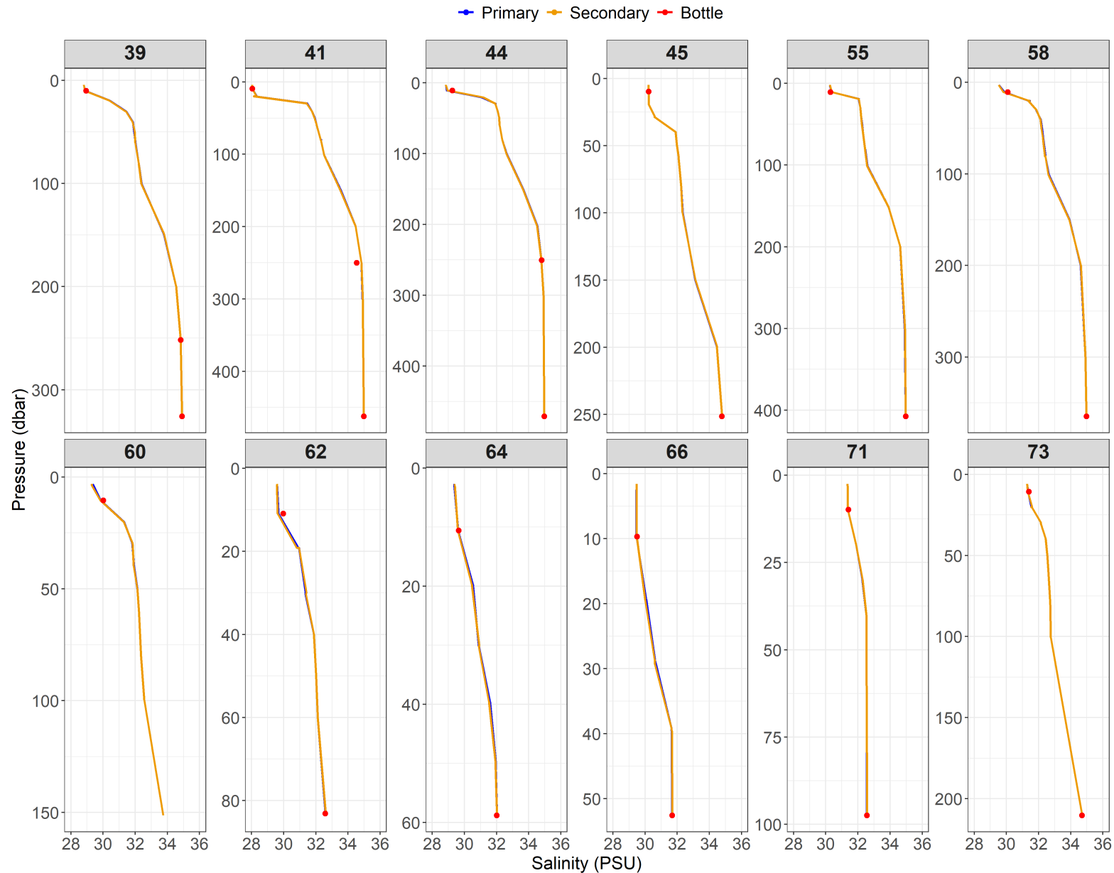
Figure A2.9: Relationship between primary (blue) and secondary (orange) salinity (from conductivity) sensor data and salinity bottle values (red) for Events 39 to 73.
