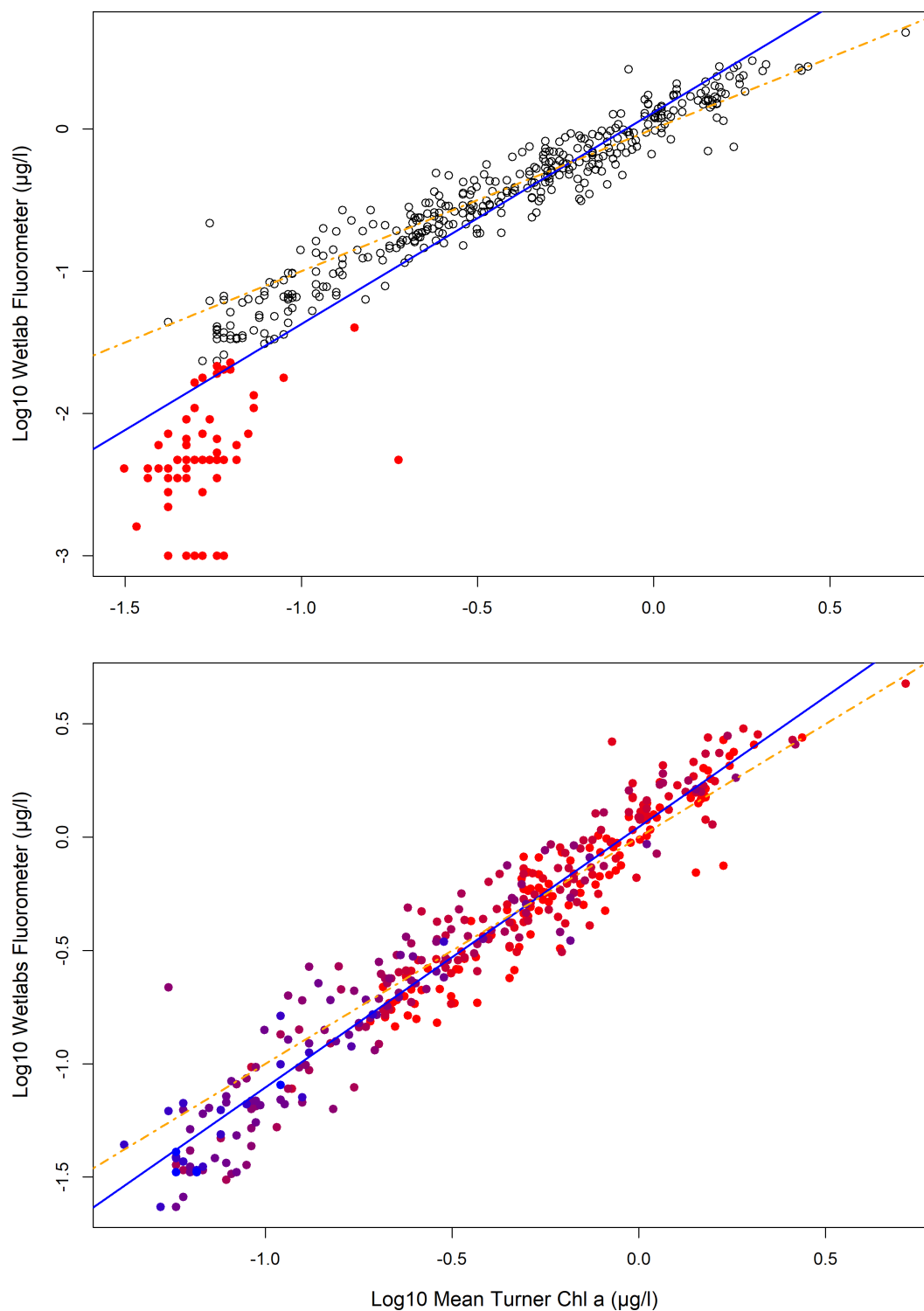
Figure A5.3: Top: log10 scale of sensor fluorometer values against mean replicate Turner fluorometer values. Outliers from Figure 5.2 are indicated in red. Bottom: log10 plot of sensor fluorometer values and replicate Turner fluorometer values (outliers removed), colour-coded by depth, where red and dark red are shallow and purple and blue are deep (closer to 100 m). In both plots, the blue line represents the line of best fit, while the orange dashed line is the 1:1 reference line.
