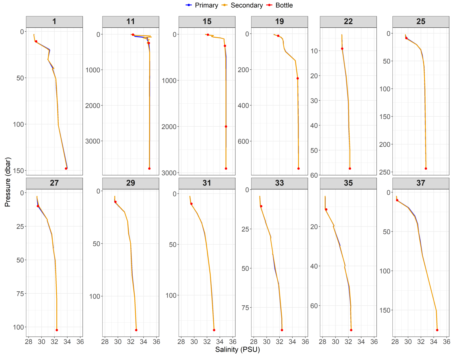
Figure A2.8: Relationship between primary (blue) and secondary (orange) salinity (from conductivity) sensor data and salinity bottle values (red) for Events 1 to 37.
