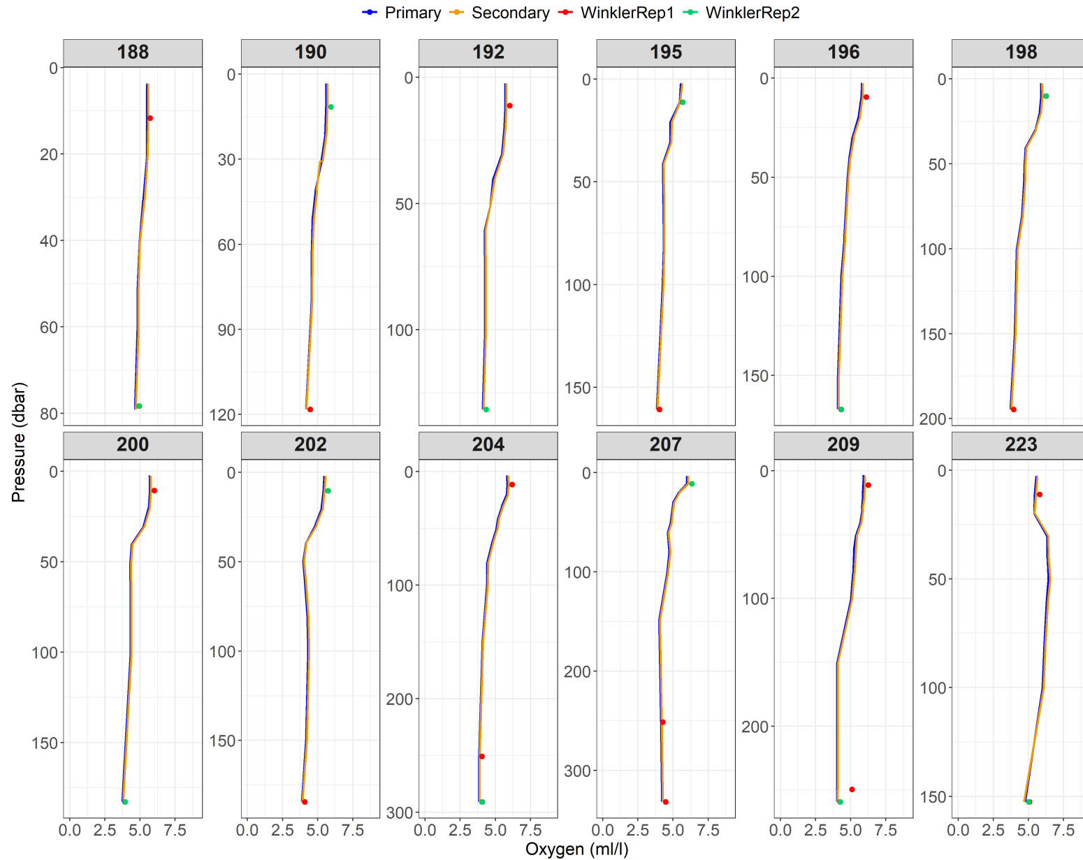
Figure A2.7: Relationship between primary (blue) and secondary (orange) dissolved oxygen sensors and dissolved oxygen measurements (replicate 1 = red, replicate 2 = green) from the Winkler titration method for Events 188 to 223.
