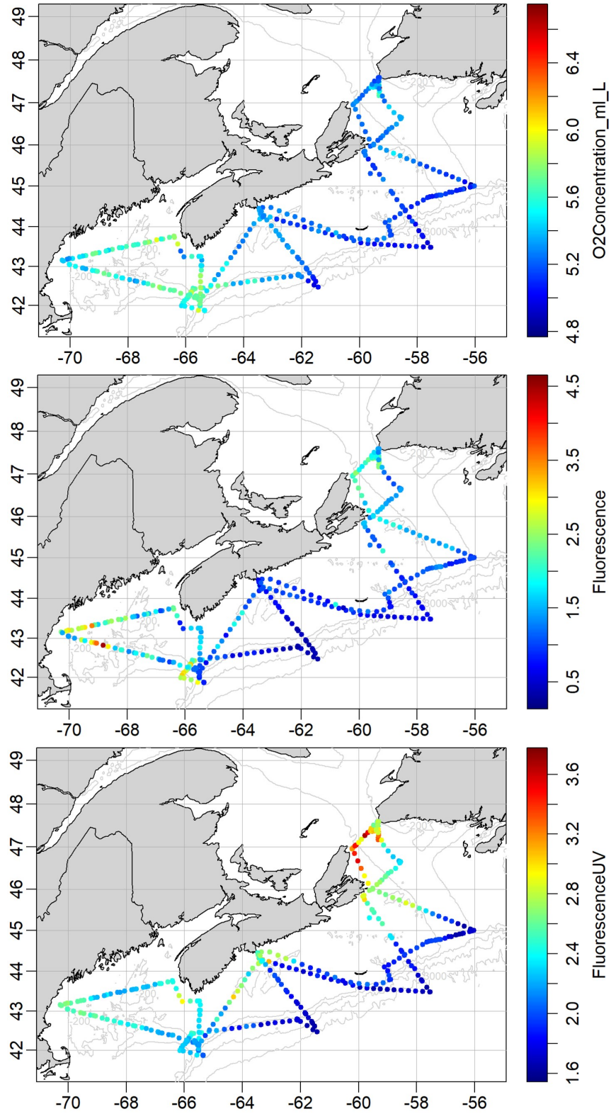
Figure 9: Dissolved oxygen concentration (ml/L; top) and chlorophyll fluorescence ( \mu\text{g/L} ; middle), and CDOM ( \mu\text{g/L} ; bottom) measured along the cruise track during the 2023 fall AZMP mission (DY16902). Data are measured at variable intervals and presented as hourly interpolations.
