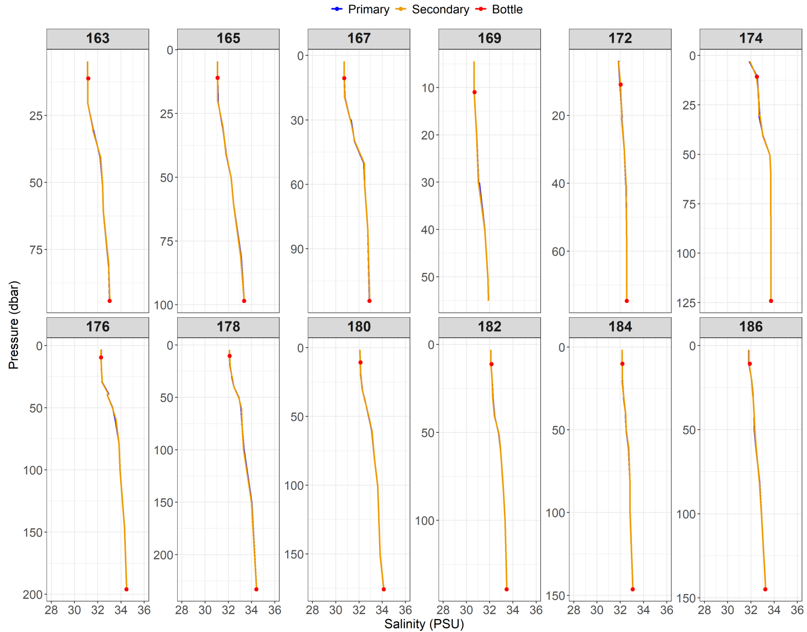
Figure A2.13: Relationship between primary (blue) and secondary (orange) salinity (from conductivity) sensor data and salinity bottle values (red) for Events 163 to 186.
