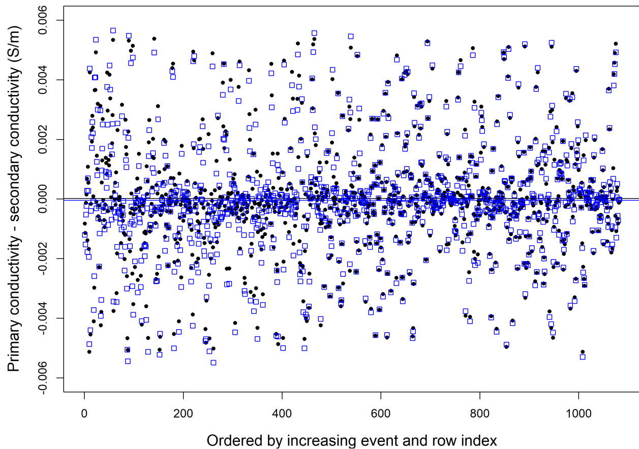
Figure A4.4: Difference between corrected (blue) versus uncorrected (black) conductivity sensor data collected on the DY16902 mission. Outliers (316) between sensors have been removed. Black dots represent the difference between uncorrected primary and secondary conductivity sensors (mean \pm SD = 1.9582 \times 10^{-5} \pm 0.0019 S/m), while blue squares represent the difference between the corrected primary and secondary sensors (mean \pm SD = -4.5253 \times 10^{-5} \pm 0.0019 S/m).
