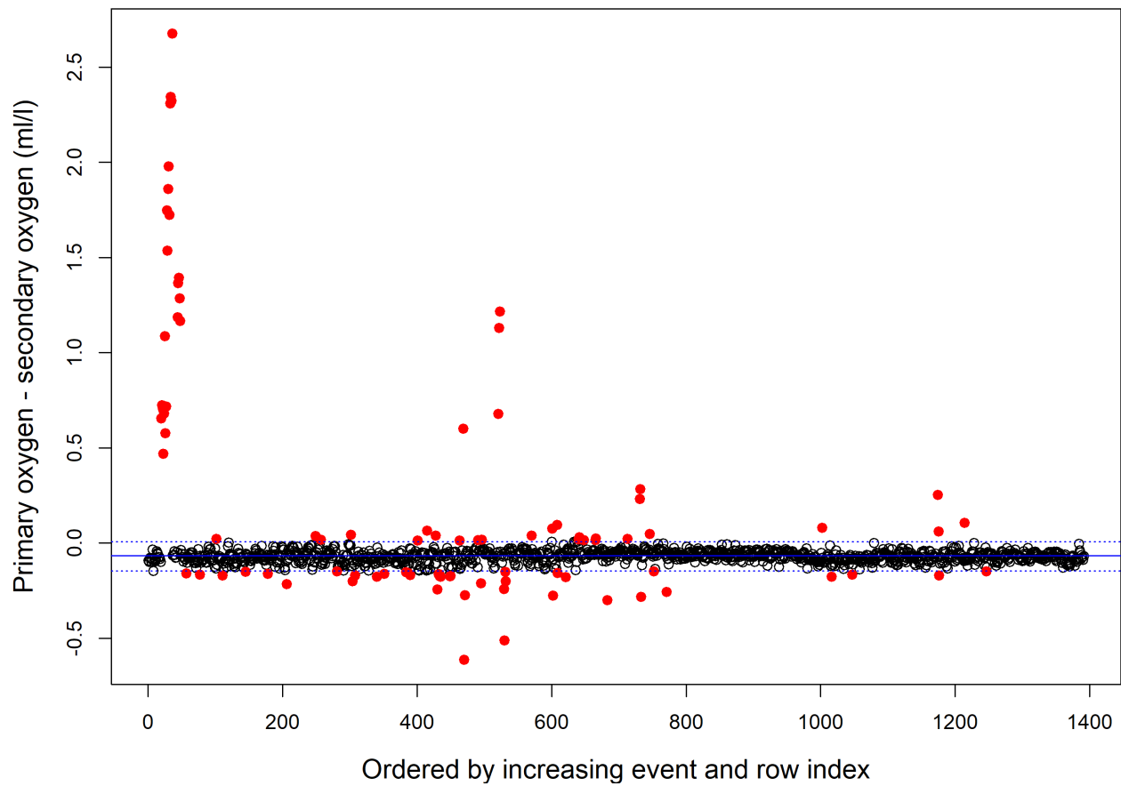
Figure A3.3: Difference between primary and secondary oxygen sensor values collected during the 2023 fall AZMP mission (DY16902). Differences outside 1.5 \times \text{IQR} (horizontal dashed blue lines) are considered outliers (red dots) and were removed from the calibration process. Boxplot statistics are as follows: Median = -0.0671, IQR min = -0.1461, IQR max = 0.0078.
