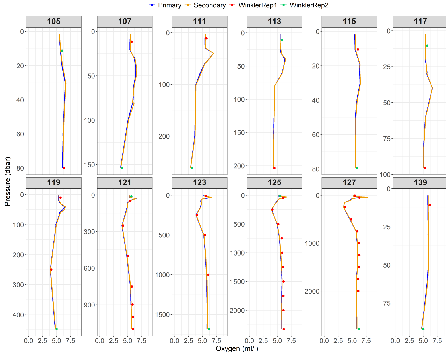
Figure A2.4: Relationship between primary (blue) and secondary (orange) dissolved oxygen sensors and dissolved oxygen measurements (replicate 1 = red, replicate 2 = green) from the Winkler titration method for Events 105 to 139.
