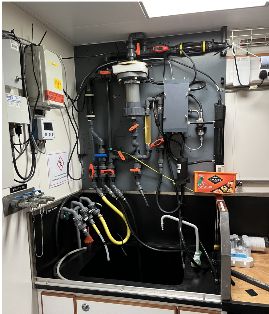
Figure 6: Ship-board underway system installed on the RRS Discovery .
