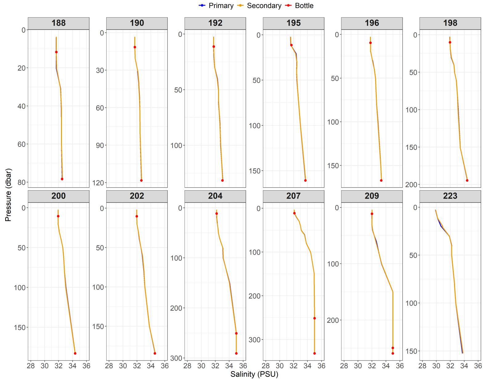
Figure A2.14: Relationship between primary (blue) and secondary (orange) salinity (from conductivity) sensor data and salinity bottle values (red) for Events 188 to 223.
