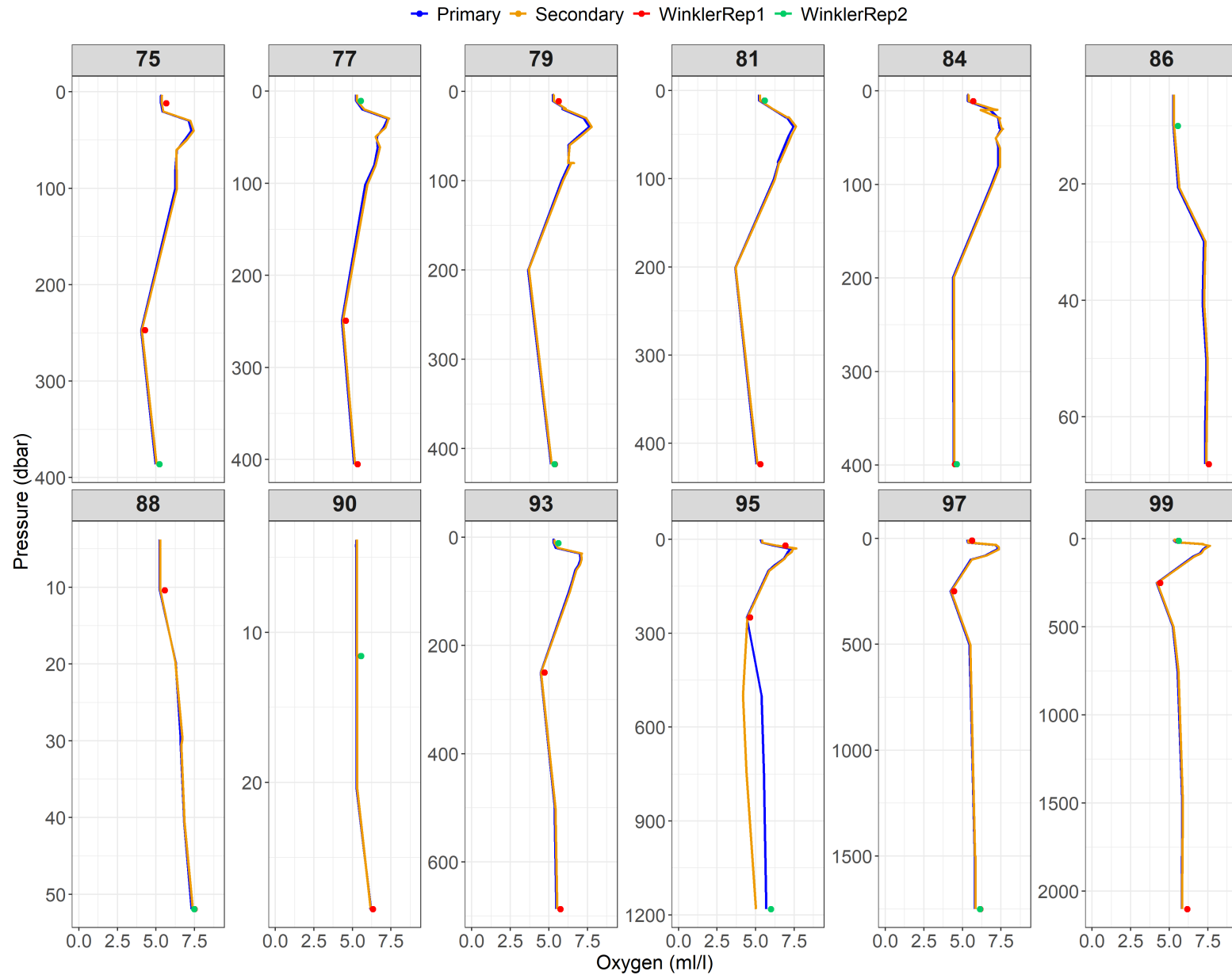
Figure A2.3: Relationship between primary (blue) and secondary (orange) dissolved oxygen sensors and dissolved oxygen measurements (replicate 1 = red, replicate 2 = green) from the Winkler titration method for Events 75 to 99.
