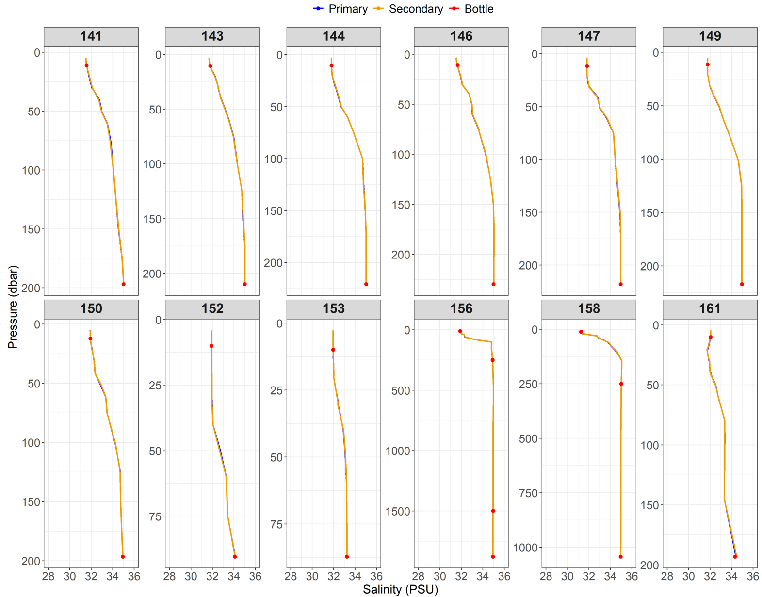
Figure A2.12: Relationship between primary (blue) and secondary (orange) salinity (from conductivity) sensor data and salinity bottle values (red) for Events 141 to 161.
