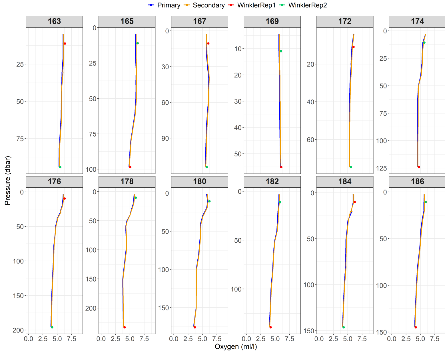
Figure A2.6: Relationship between primary (blue) and secondary (orange) dissolved oxygen sensors and dissolved oxygen measurements (replicate 1 = red, replicate 2 = green) from the Winkler titration method for Events 163 to 186.
