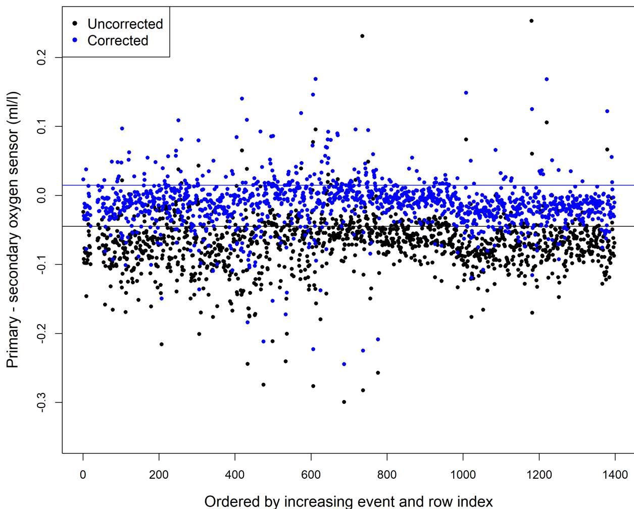
Figure A3.6: Difference in the primary and secondary sensor values of the uncorrected (black) and corrected (blue) data collected during the 2023 fall AZMP mission (DY16902). All data (including outliers removed in the above processes) were corrected. The black and blue lines represent the mean difference between the primary and secondary sensors for the uncorrected (black) and corrected (blue) data, respectively.
