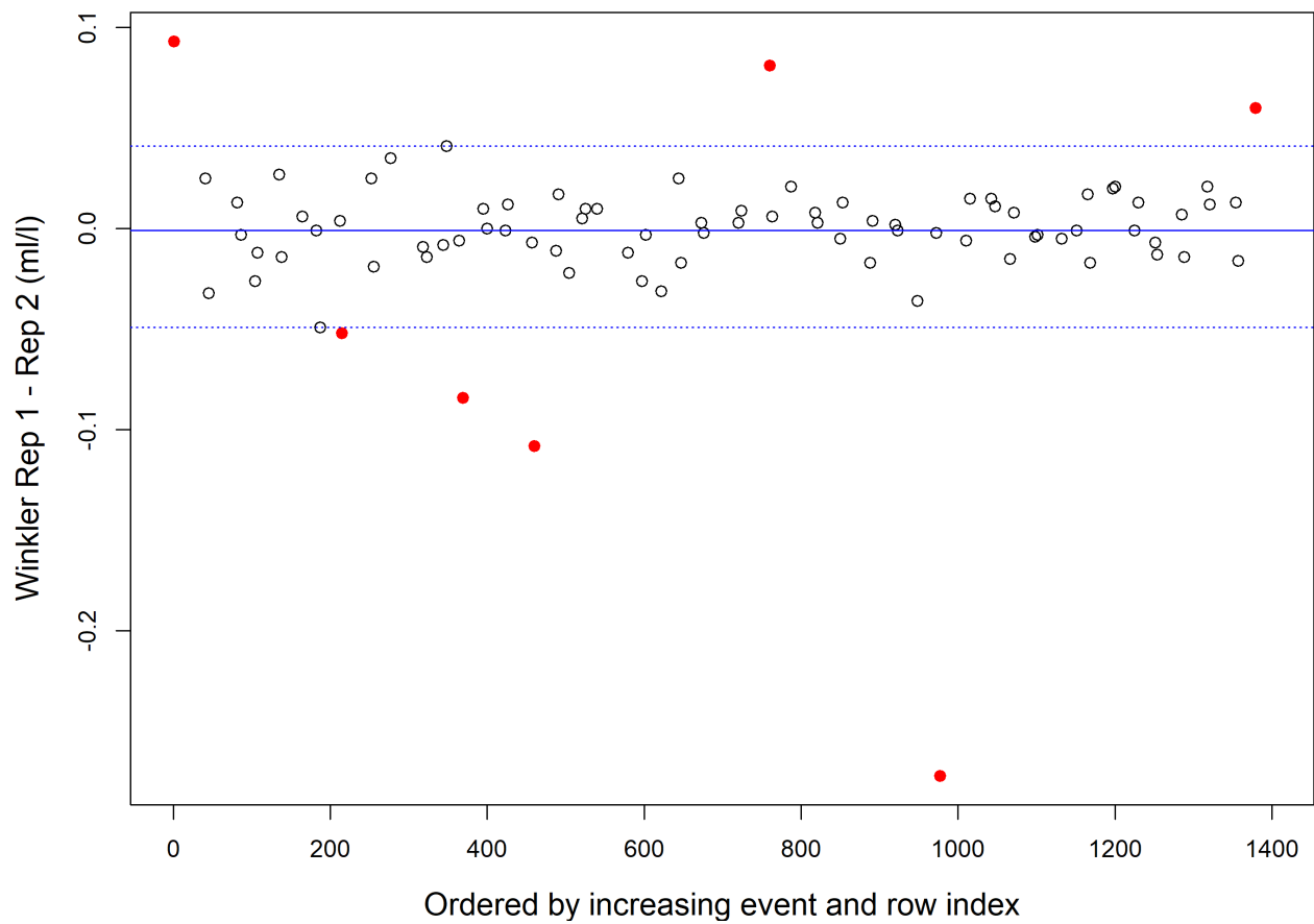
Figure A3.2: Comparison of Winkler replicates measured during the 2023 fall AZMP mission (DY16902). Differences outside 1.5*IQR (horizontal dashed blue lines) are considered outliers (red dots) and were removed from the calibration process. Boxplot statistics are as follows: Median = -0.0010, IQR min = -0.0490, IQR max = 0.0410.
