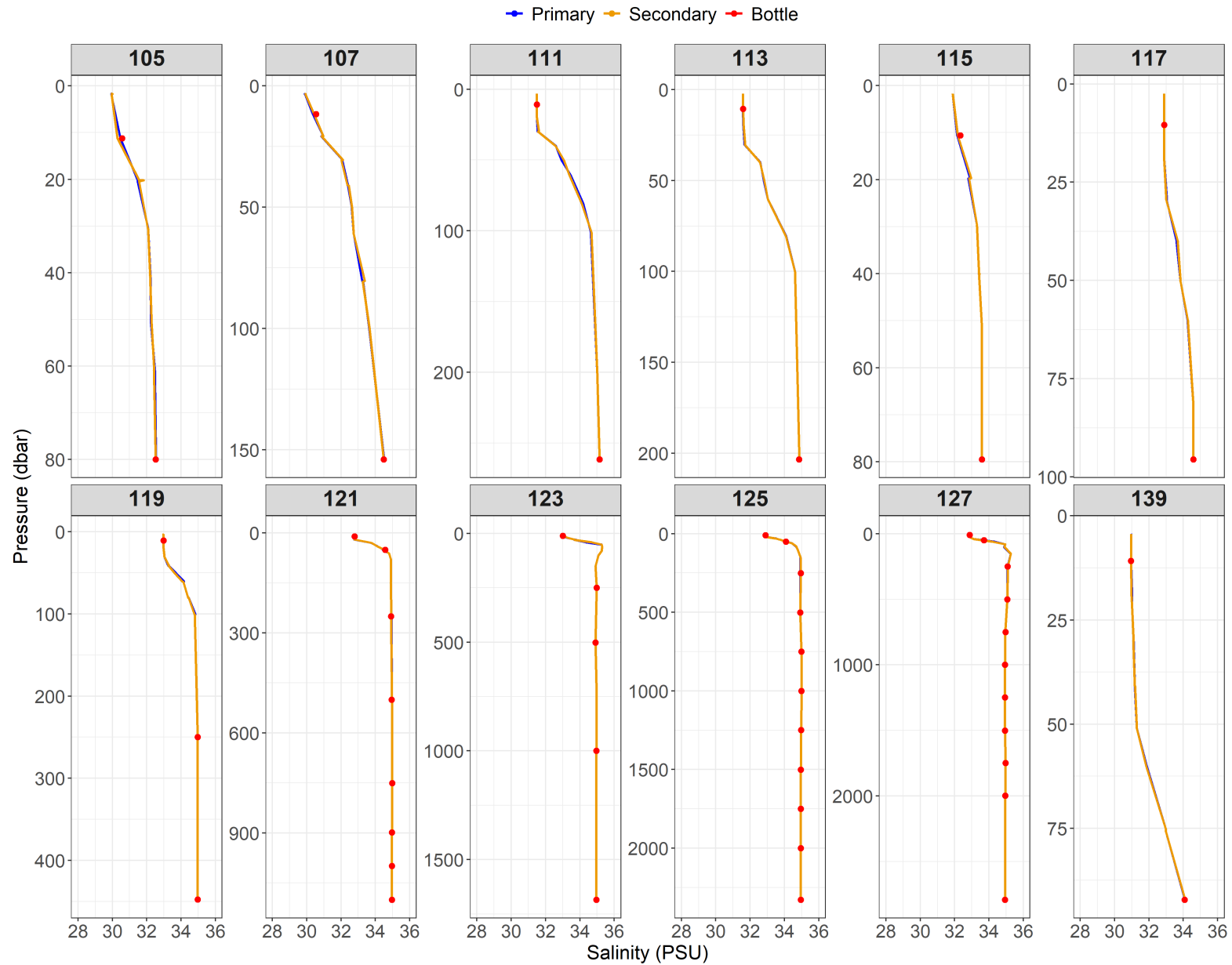
Figure A2.11: Relationship between primary (blue) and secondary (orange) salinity (from conductivity) sensor data and salinity bottle values (red) for Events 105 to 139.
