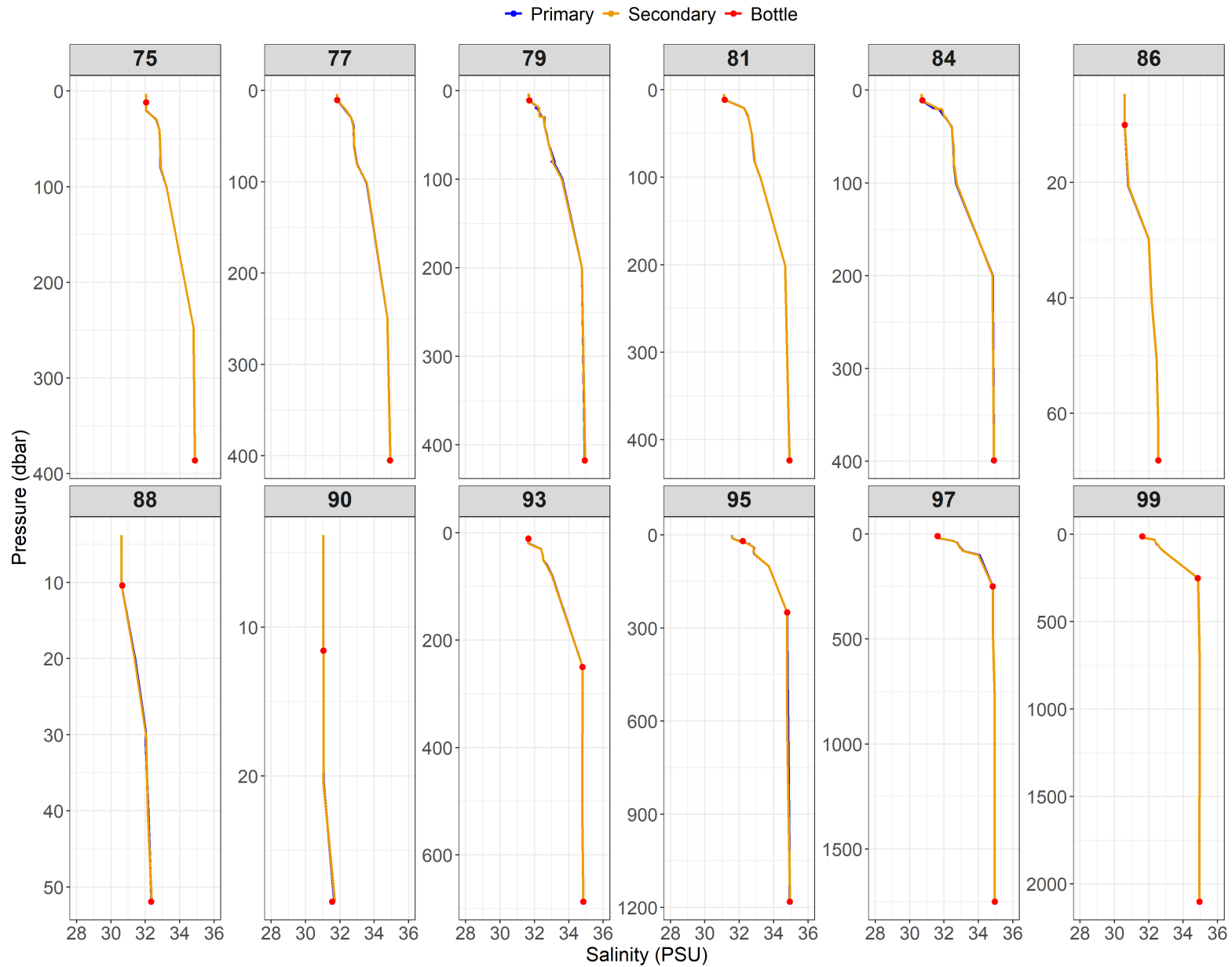
Figure A2.10: Relationship between primary (blue) and secondary (orange) salinity (from conductivity) sensor data and salinity bottle values (red) for Events 75 to 99.
