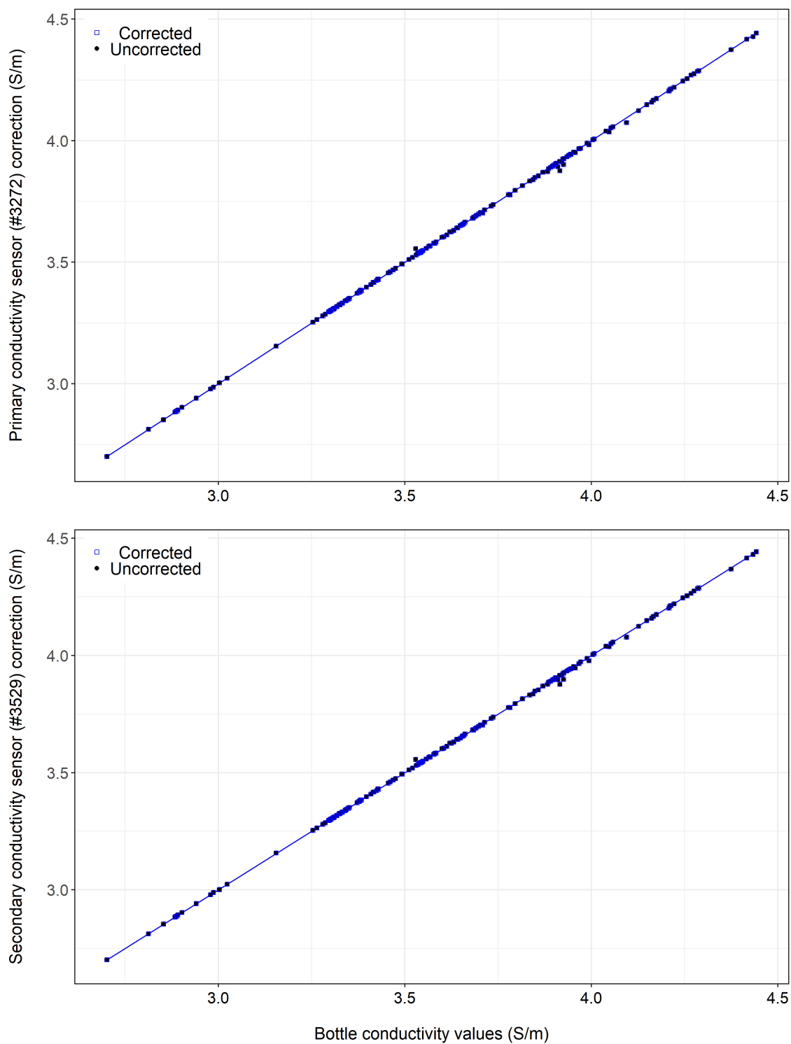
Figure A4.5: Primary (top) and secondary (bottom) conductivity sensor data before (black dots) and after (blue squares) correction using the determined slopes and offsets. The blue line represents the 1:1 reference line of the corrected data.
